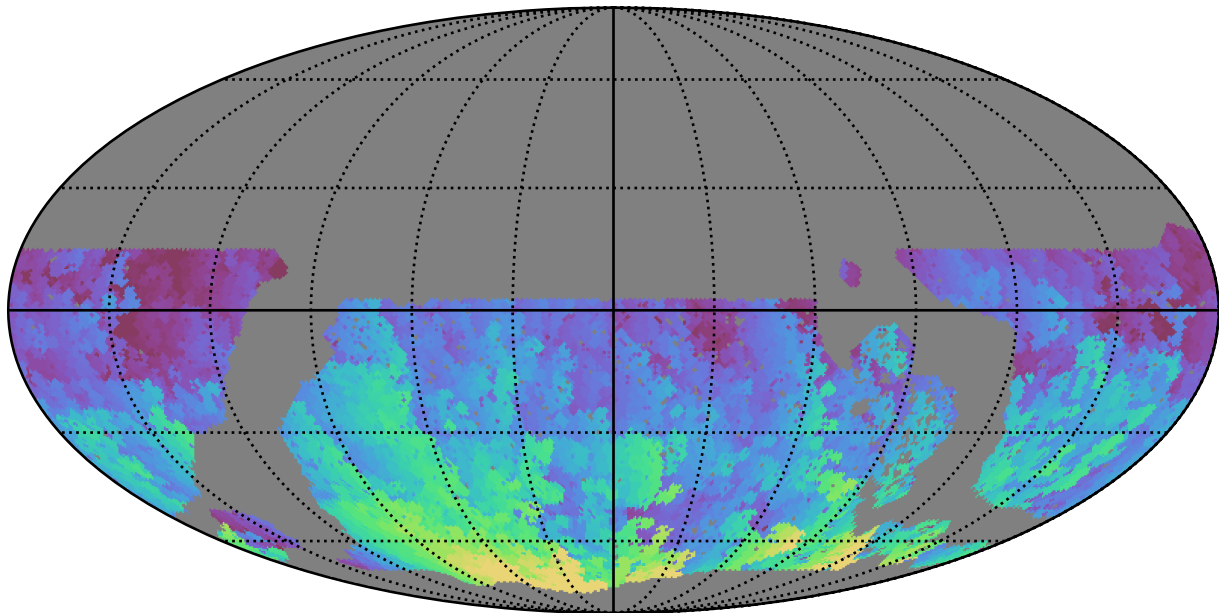
roll_pause_mjdp60_v3.4_10yrs WFD u band: Max HA
