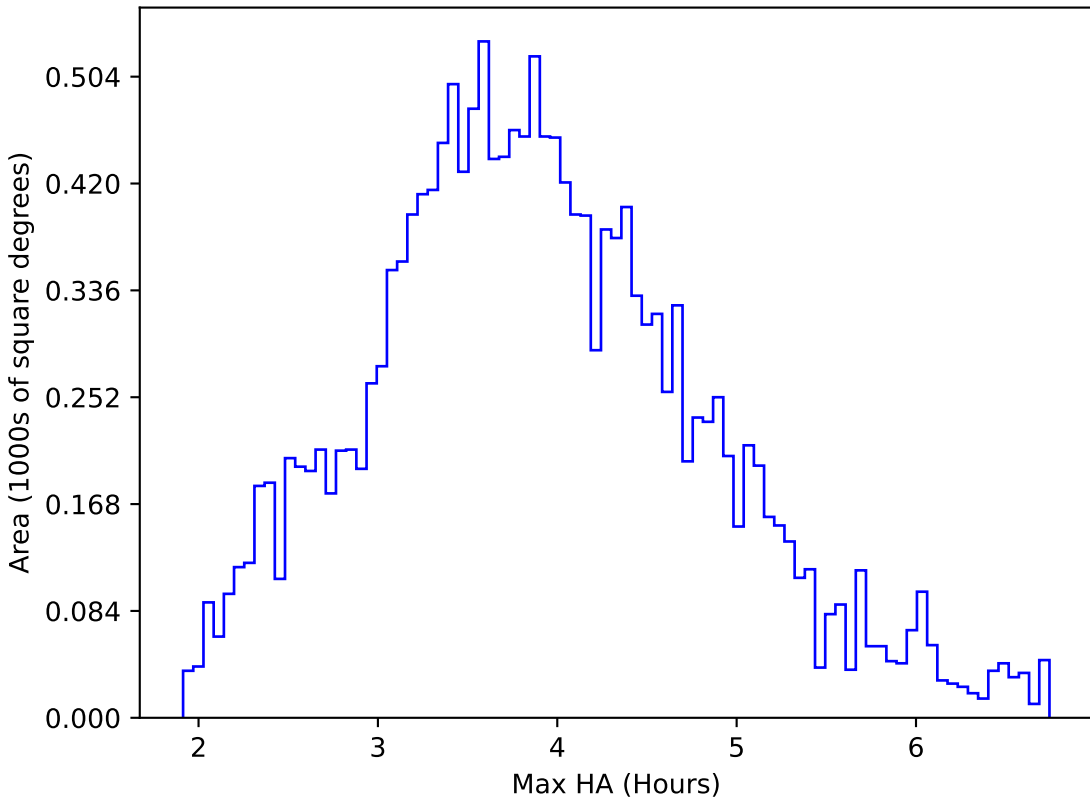
roll_pause_mjdp60_v3.4_10yrs WFD u band: Max HA
