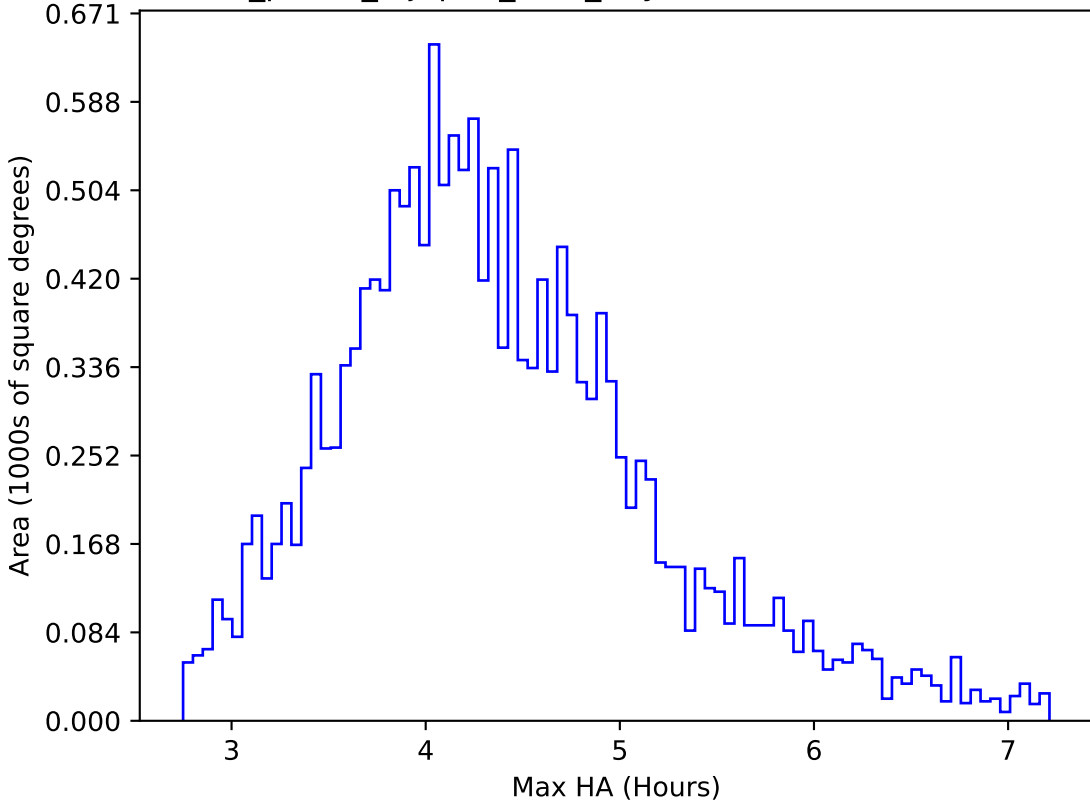
roll_pause_mjdp60_v3.4_10yrs WFD r band: Max HA
