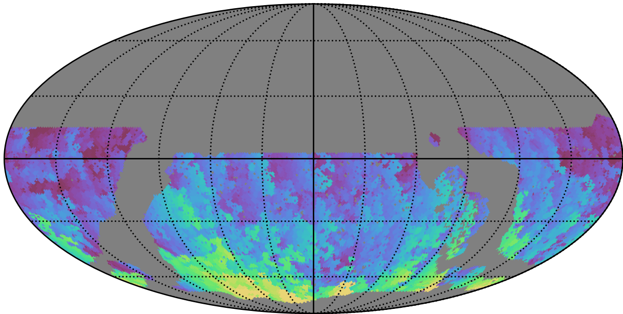
roll_pause_mjdp60_v3.4_10yrs WFD g band: Max HA
