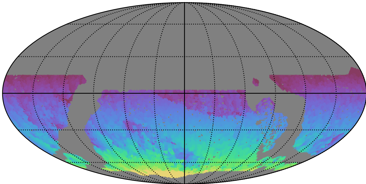
roll_pause_mjdp60_v3.4_10yrs WFD all bands: Max HA
