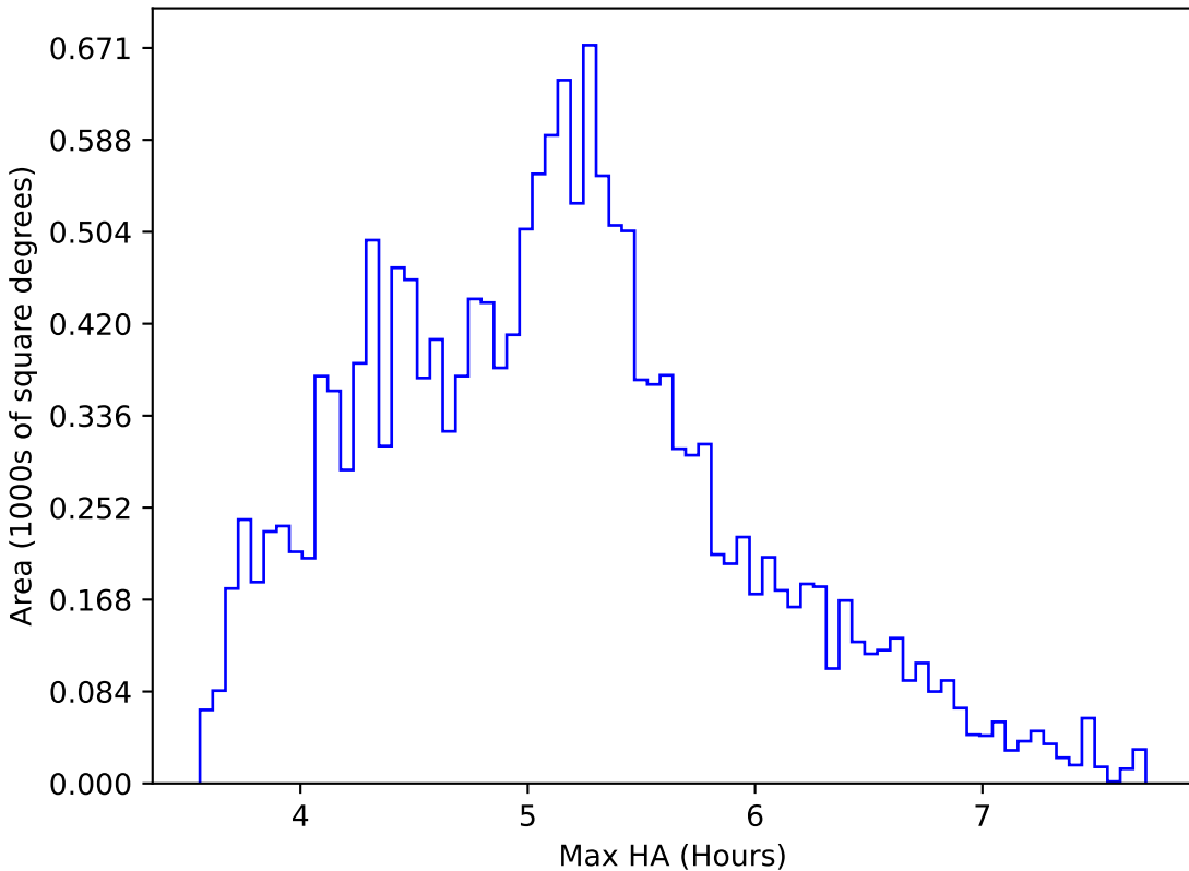
roll_pause_mjdp60_v3.4_10yrs WFD all bands: Max HA
