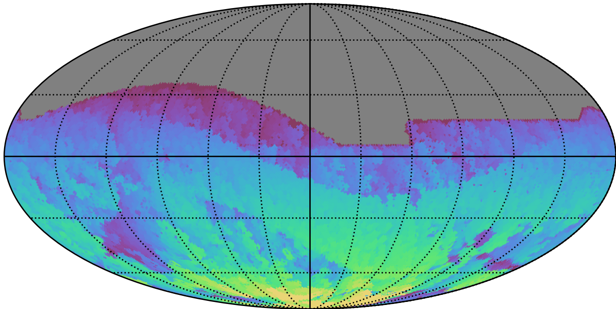
roll_pause_mjdp60_v3.4_10yrs All sky z band: Max HA
