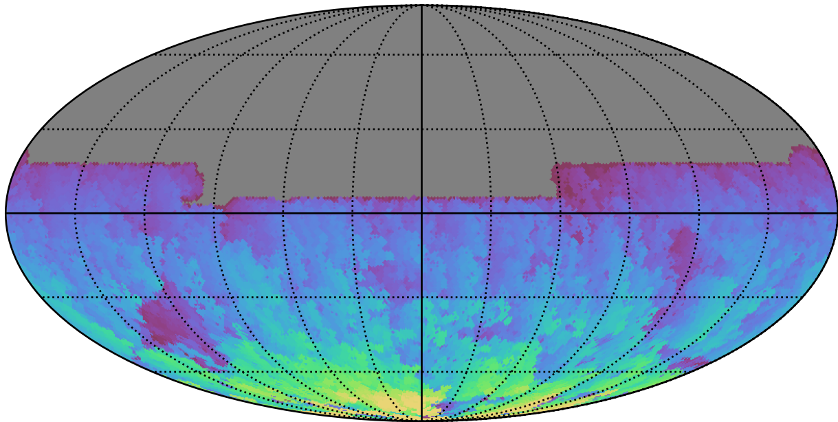
roll_pause_mjdp60_v3.4_10yrs All sky y band: Max HA
