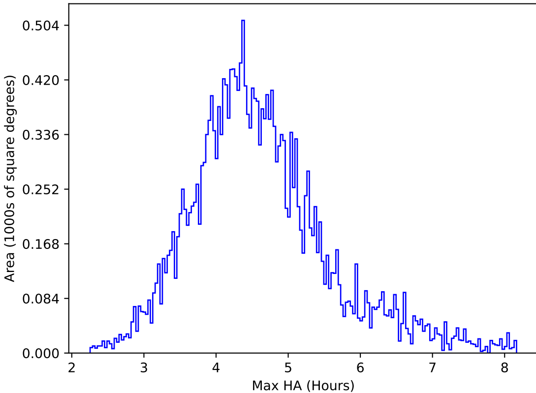
roll_pause_mjdp60_v3.4_10yrs All sky y band: Max HA
