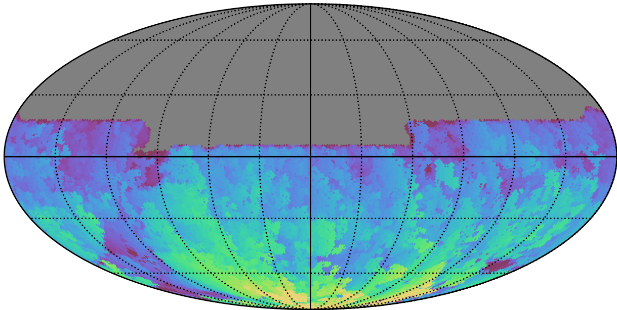
roll_pause_mjdp60_v3.4_10yrs All sky u band: Max HA
