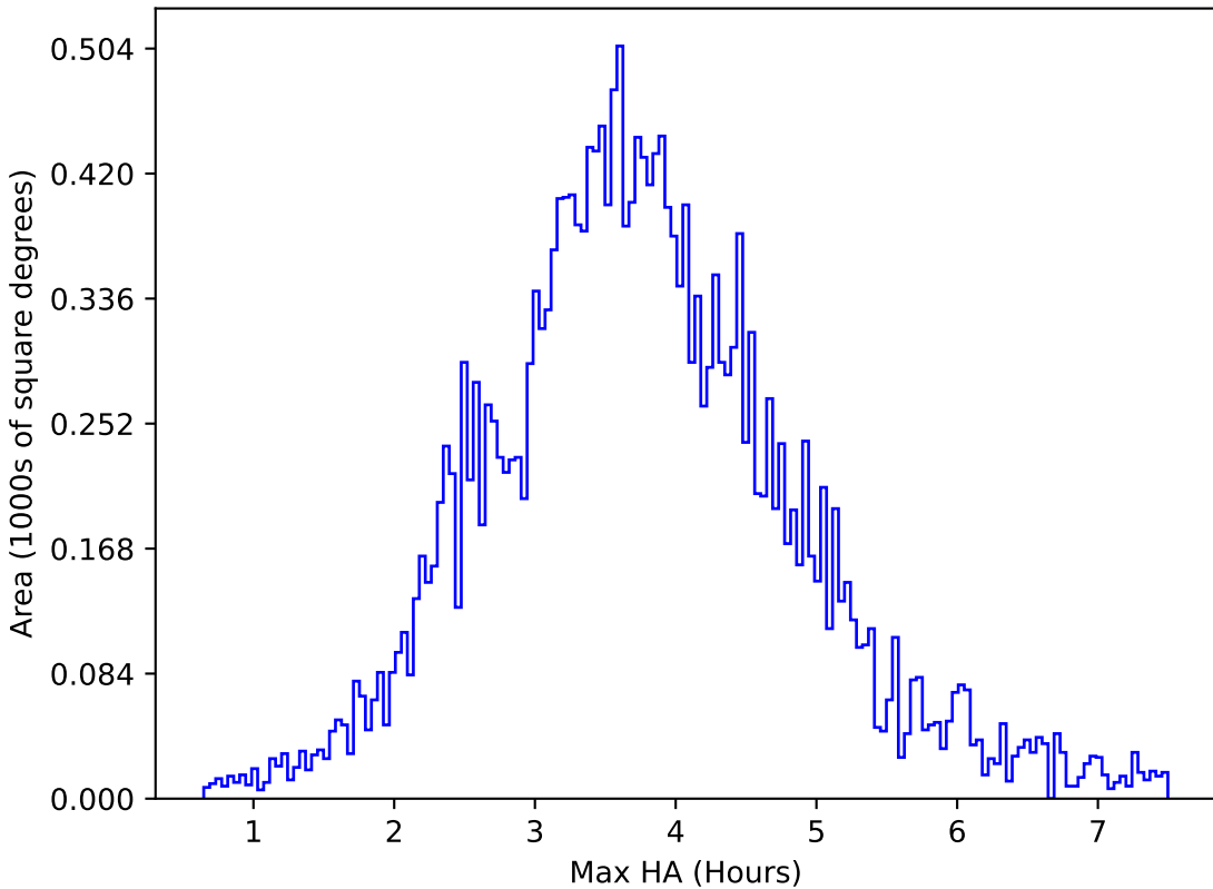
roll_pause_mjdp60_v3.4_10yrs All sky u band: Max HA
