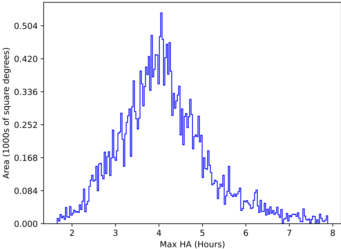
roll_pause_mjdp60_v3.4_10yrs All sky r band: Max HA
