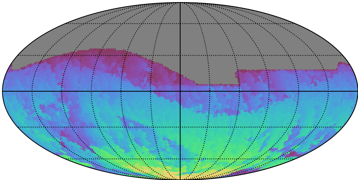
roll_pause_mjdp60_v3.4_10yrs All sky i band: Max HA
