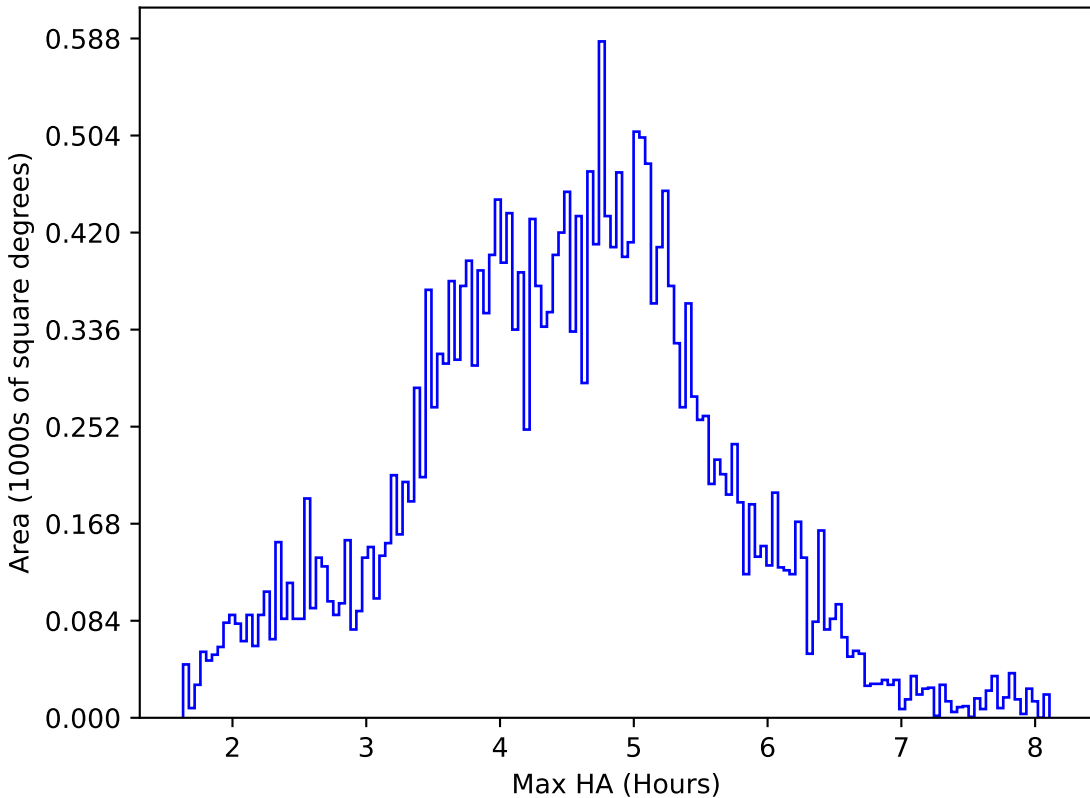
roll_pause_mjdp60_v3.4_10yrs All sky i band: Max HA
