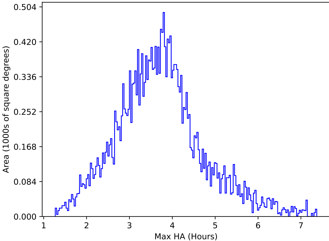
roll_pause_mjdp60_v3.4_10yrs All sky g band: Max HA
