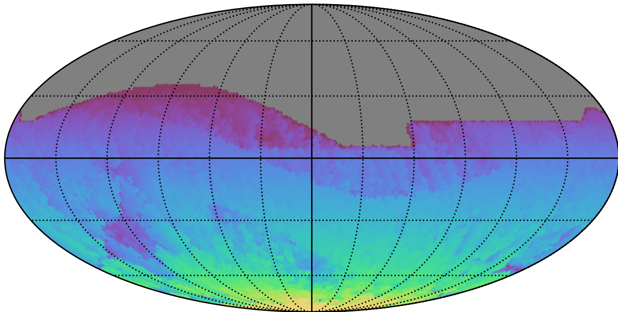
roll_pause_mjdp60_v3.4_10yrs All sky all bands: Max HA
