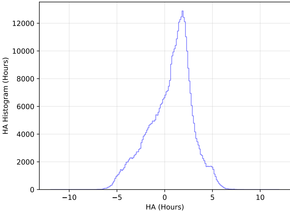
roll_pause_mjdp60_v3.4_10yrs WFD z band: HA Histogram
