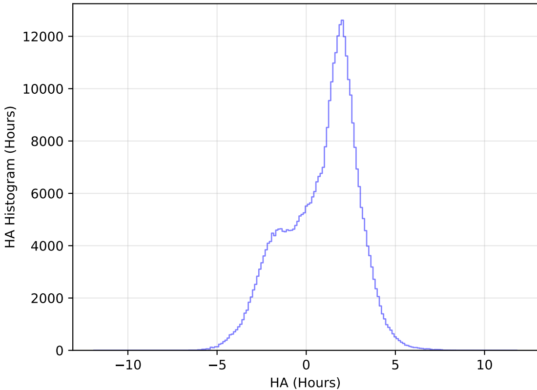
roll_pause_mjdp60_v3.4_10yrs WFD y band: HA Histogram
