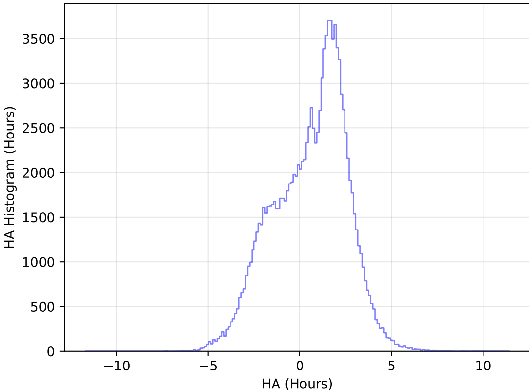
roll_pause_mjdp60_v3.4_10yrs WFD u band: HA Histogram
