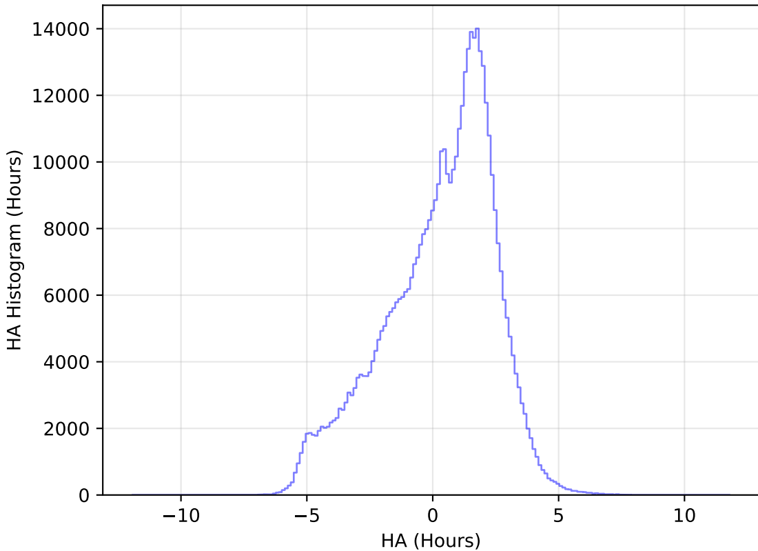
roll_pause_mjdp60_v3.4_10yrs WFD r band: HA Histogram
