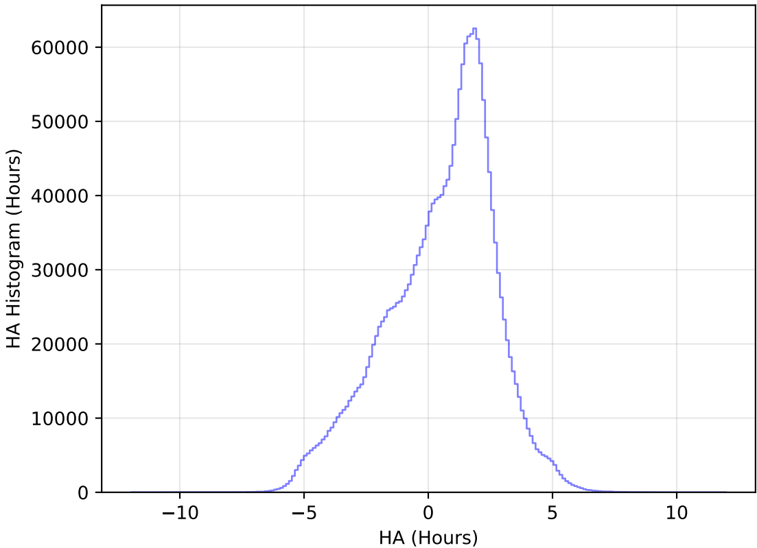
roll_pause_mjdp60_v3.4_10yrs WFD all bands: HA Histogram
