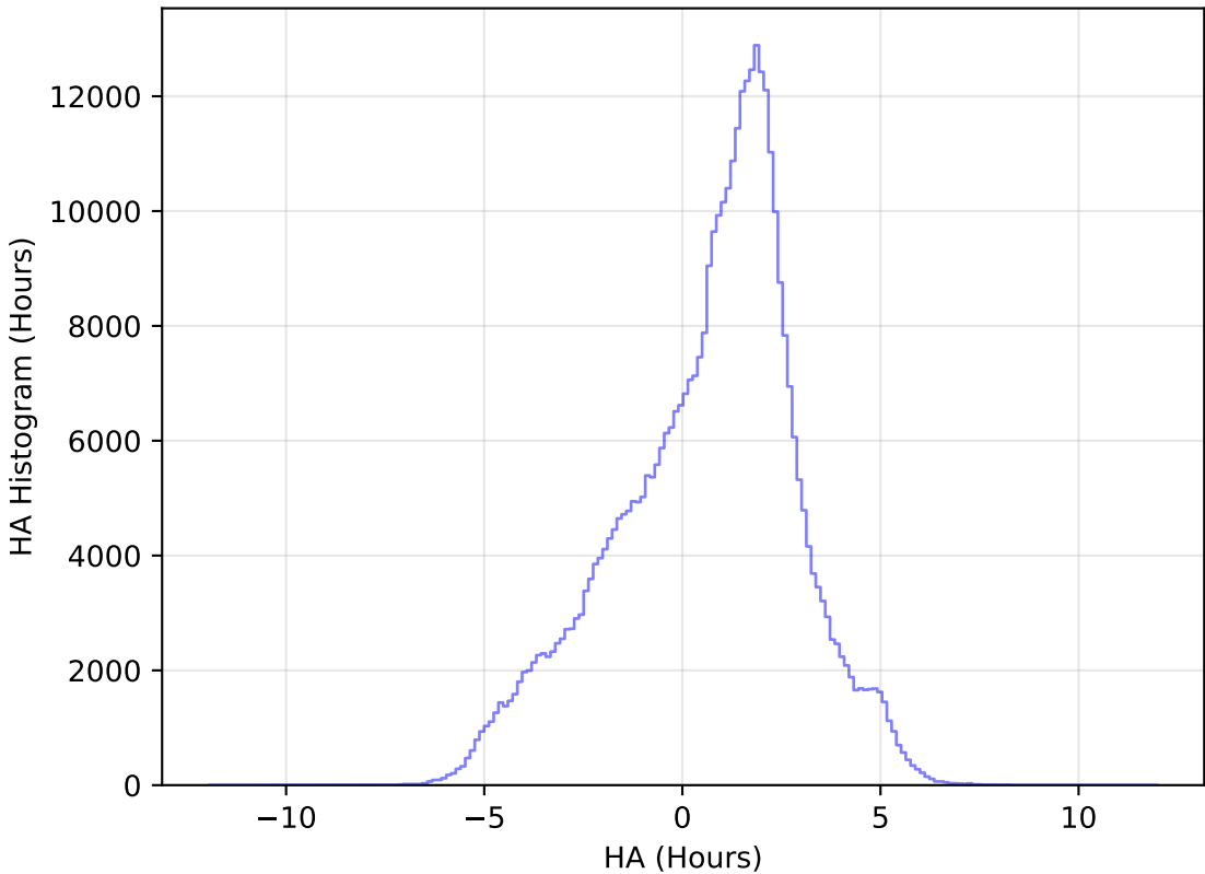
roll_pause_mjdp60_v3.4_10yrs All sky z band: HA Histogram
