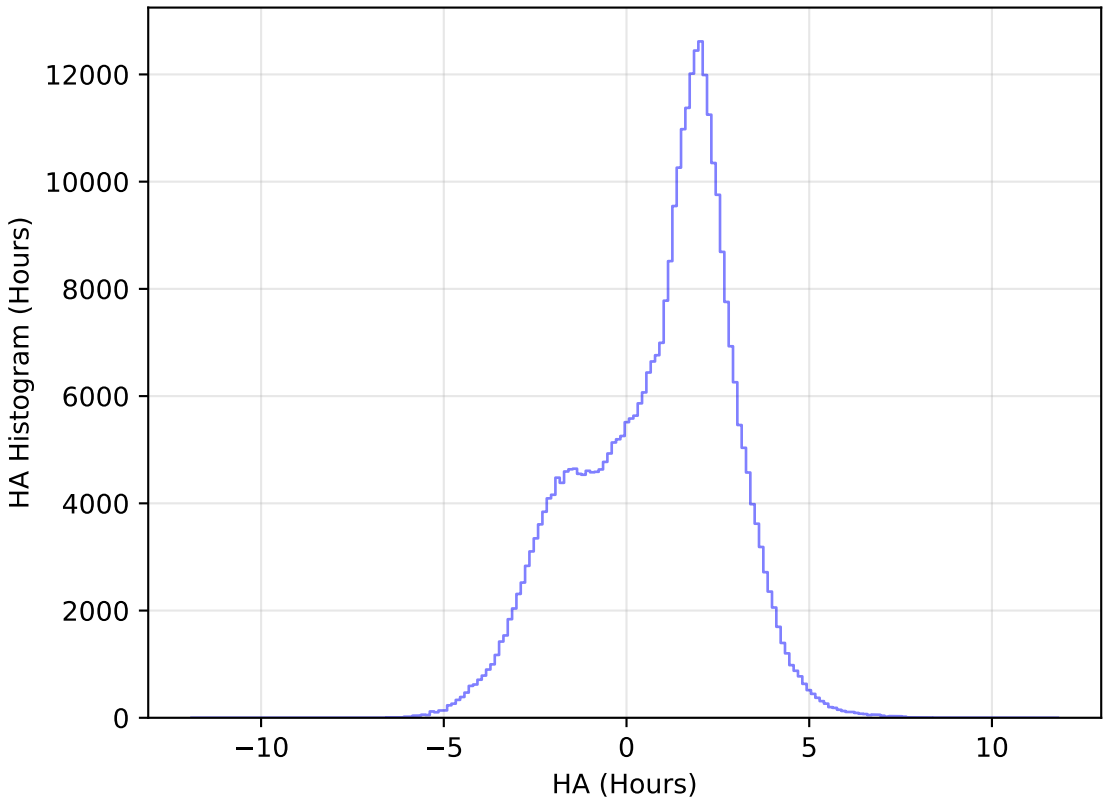
roll_pause_mjdp60_v3.4_10yrs All sky y band: HA Histogram
