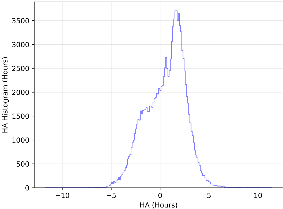
roll_pause_mjdp60_v3.4_10yrs All sky u band: HA Histogram
