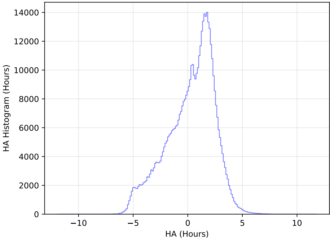
roll_pause_mjdp60_v3.4_10yrs All sky r band: HA Histogram
