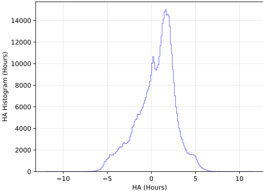
roll_pause_mjdp60_v3.4_10yrs All sky i band: HA Histogram
