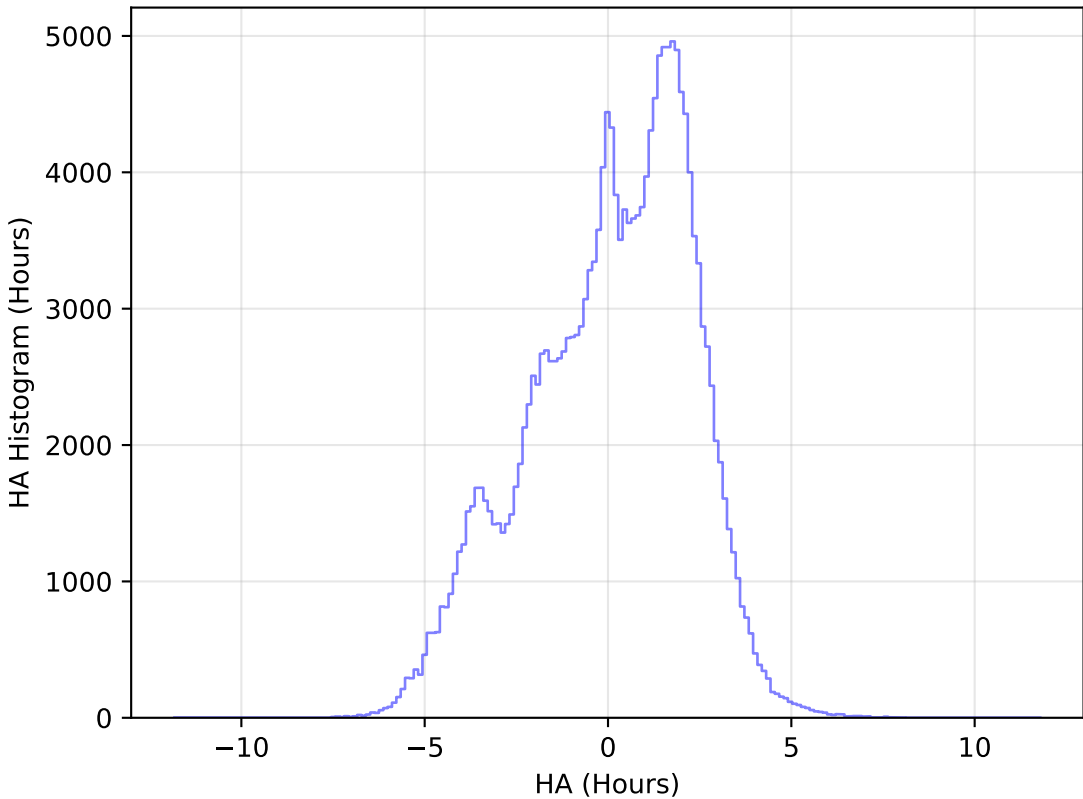
roll_pause_mjdp60_v3.4_10yrs All sky g band: HA Histogram
