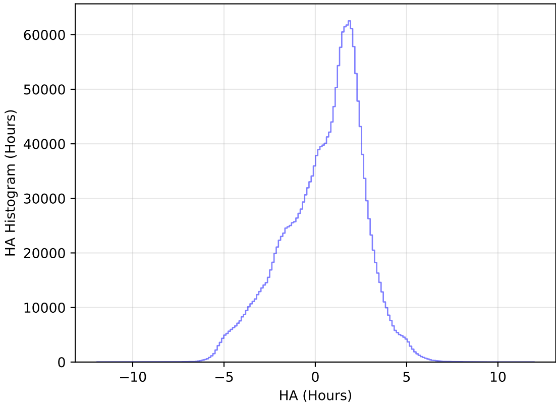
roll_pause_mjdp60_v3.4_10yrs All sky all bands: HA Histogram
