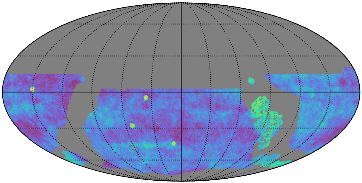
roll_pause_mjdp60_v3.4_10yrs gri WFD: Fraction of visits in pairs (20-90 min)
