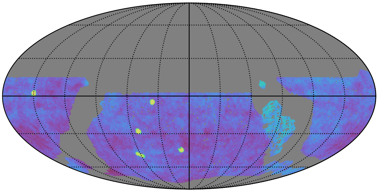
roll_pause_mjdp60_v3.4_10yrs gri WFD: Fraction of visits in pairs (10-60 min)
