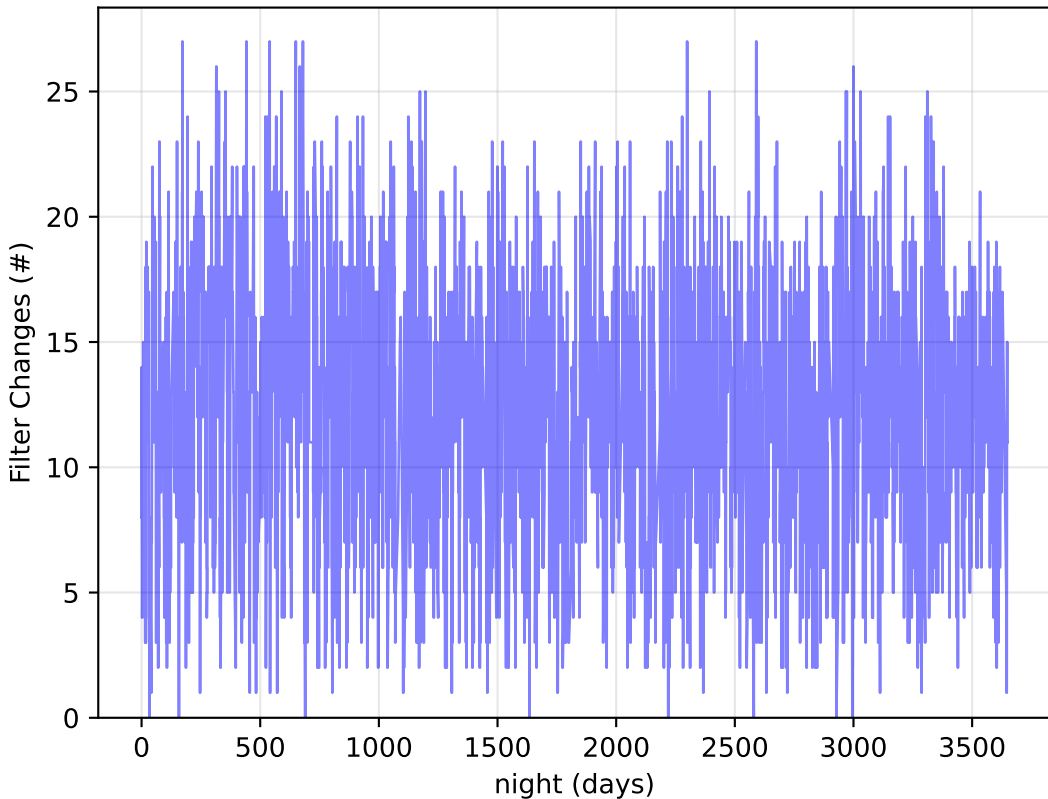
roll_pause_mjdp60_v3.4_10yrs Per Night: Filter Changes
