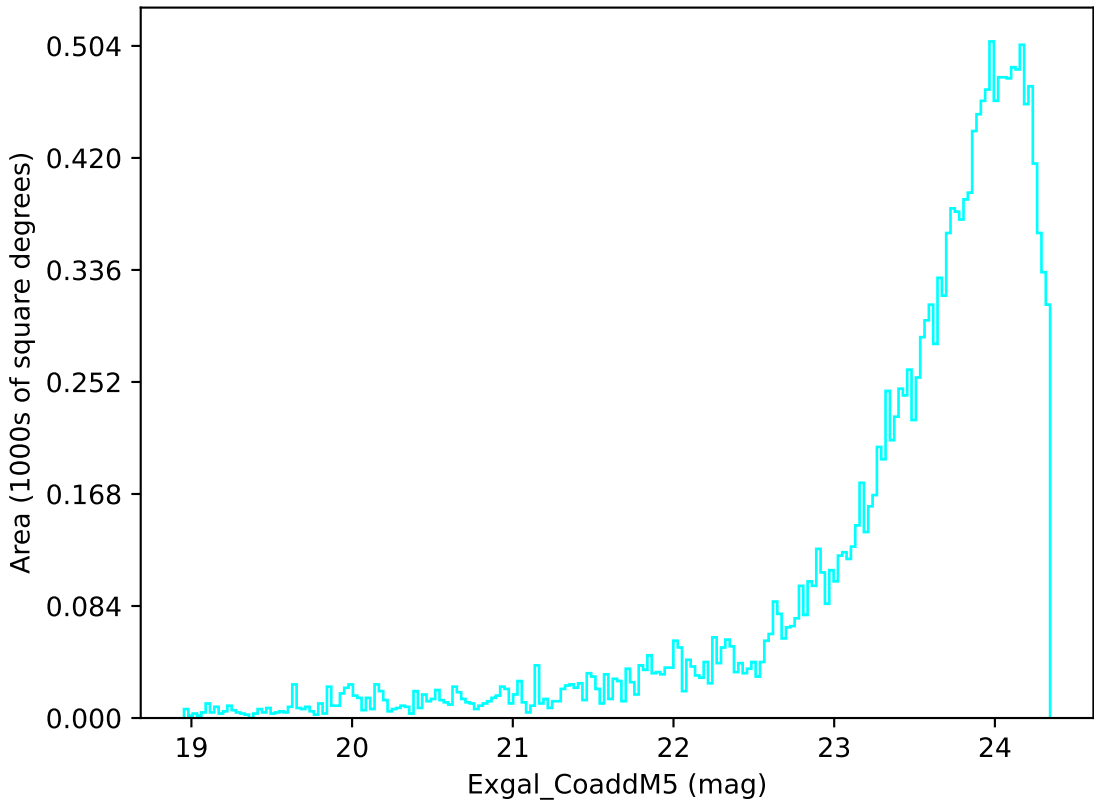
roll_pause_mjdp60_v3.4_10yrs Yr 3-4 u band: Exgal_CoaddM5
