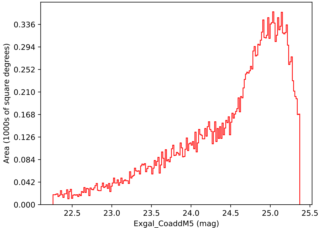
roll_pause_mjdp60_v3.4_10yrs Yr 3-4 i band: Exgal_CoaddM5
