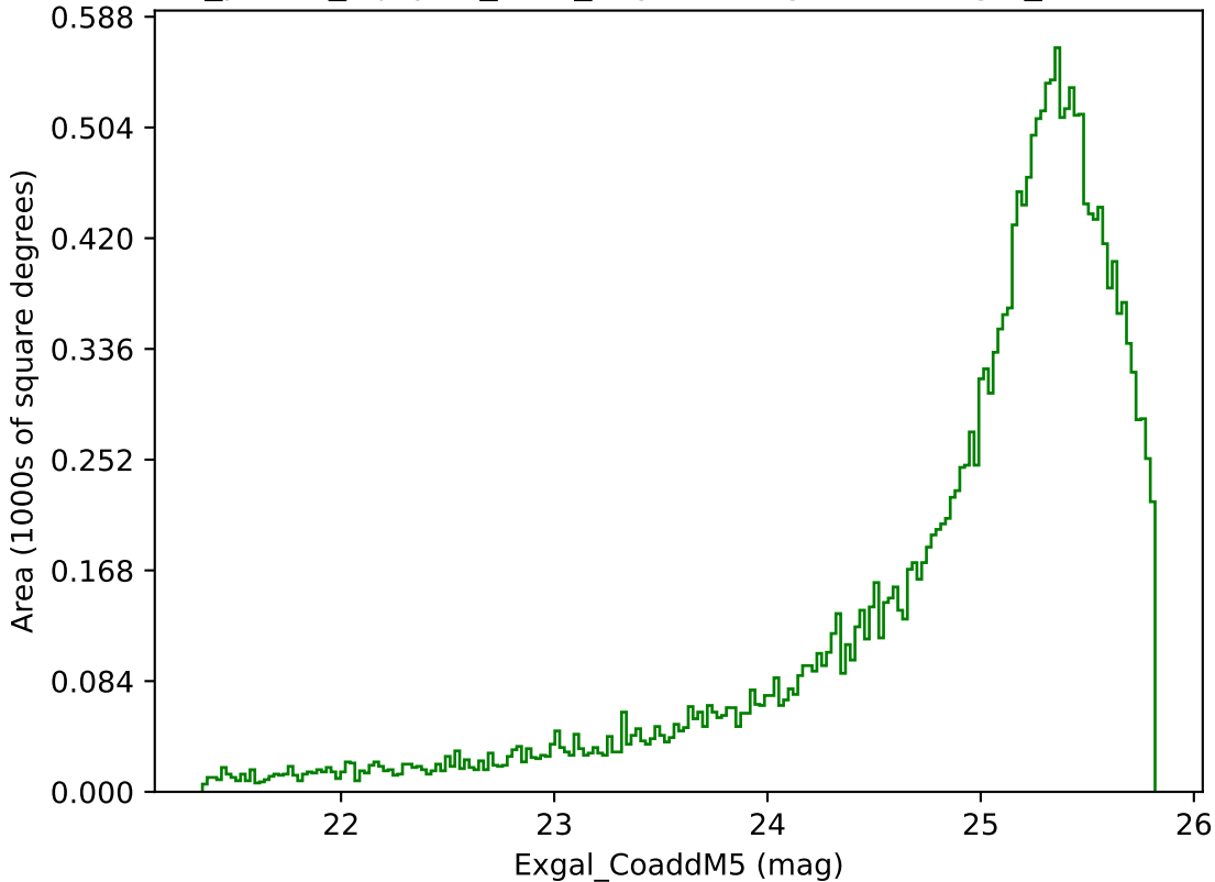
roll_pause_mjdp60_v3.4_10yrs Yr 1 g band: Exgal_CoaddM5
