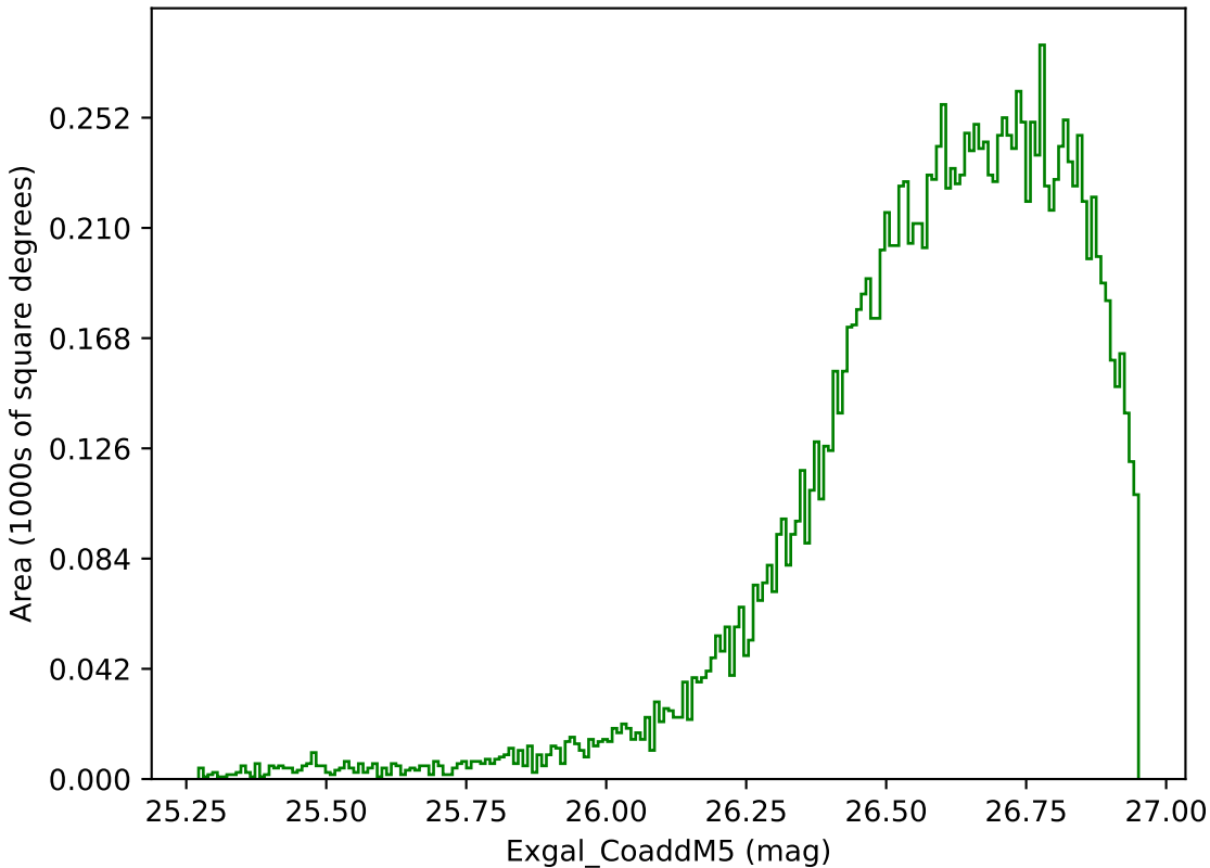
roll_pause_mjdp60_v3.4_10yrs WFD g band: Exgal_CoaddM5
