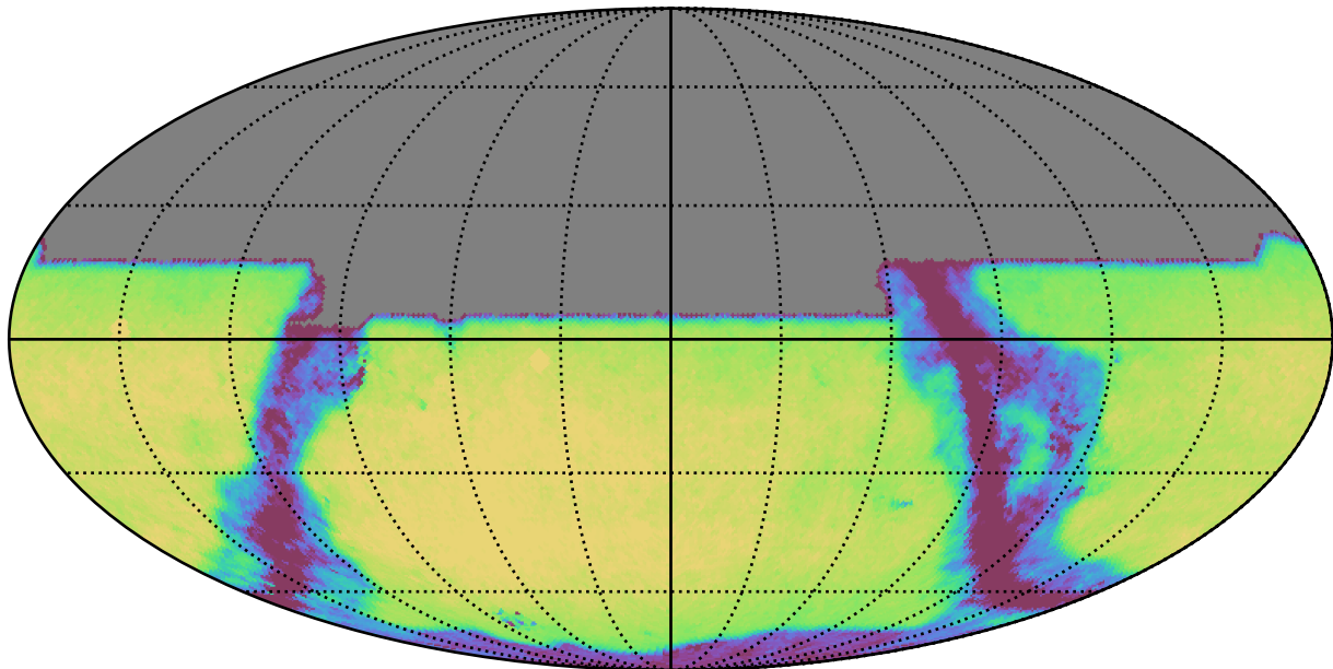
roll_pause_mjdp60_v3.4_10yrs All sky y band: Exgal_CoaddM5
