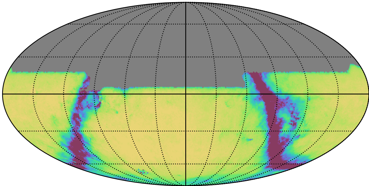
roll_pause_mjdp60_v3.4_10yrs All sky u band: Exgal_CoaddM5
