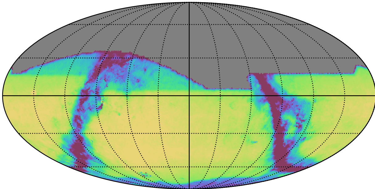
roll_pause_mjdp60_v3.4_10yrs All sky i band: Exgal_CoaddM5
