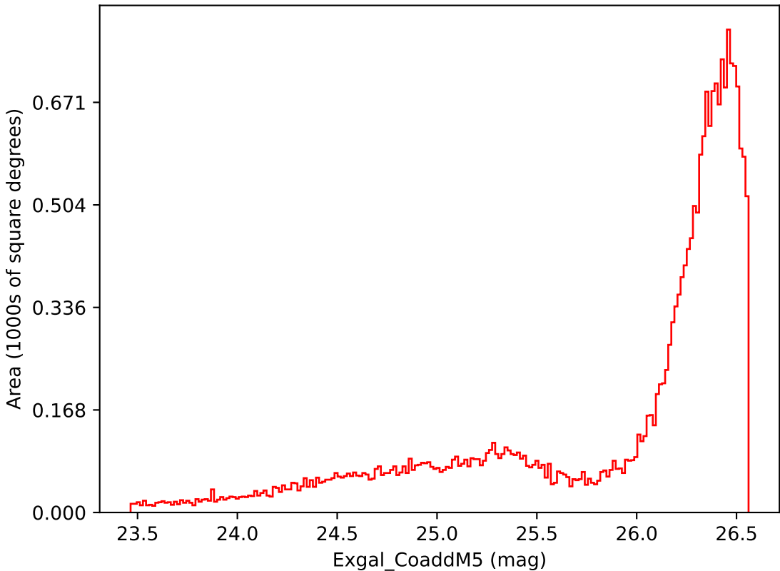
roll_pause_mjdp60_v3.4_10yrs All sky i band: Exgal_CoaddM5
