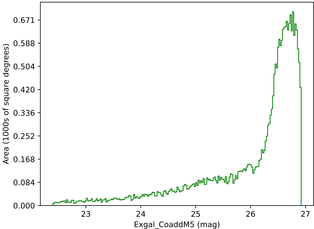
roll_pause_mjdp60_v3.4_10yrs All sky g band: Exgal_CoaddM5
