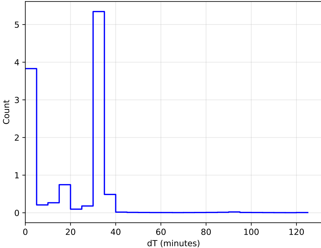
roll_pause_mjdp60_v3.4_10yrs WFD: DeltaT Histogram
