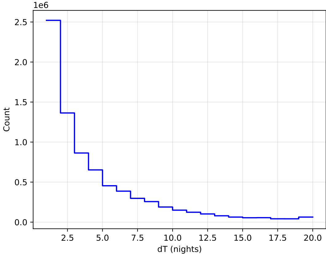
roll_pause_mjdp60_v3.4_10yrs WFD all bands: DeltaNight Histogram
