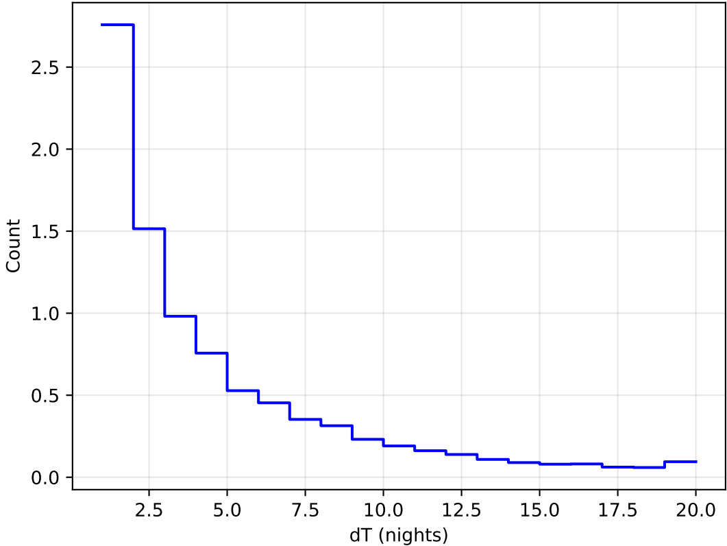
roll_pause_mjdp60_v3.4_10yrs All sky all bands: DeltaNight Histogram
