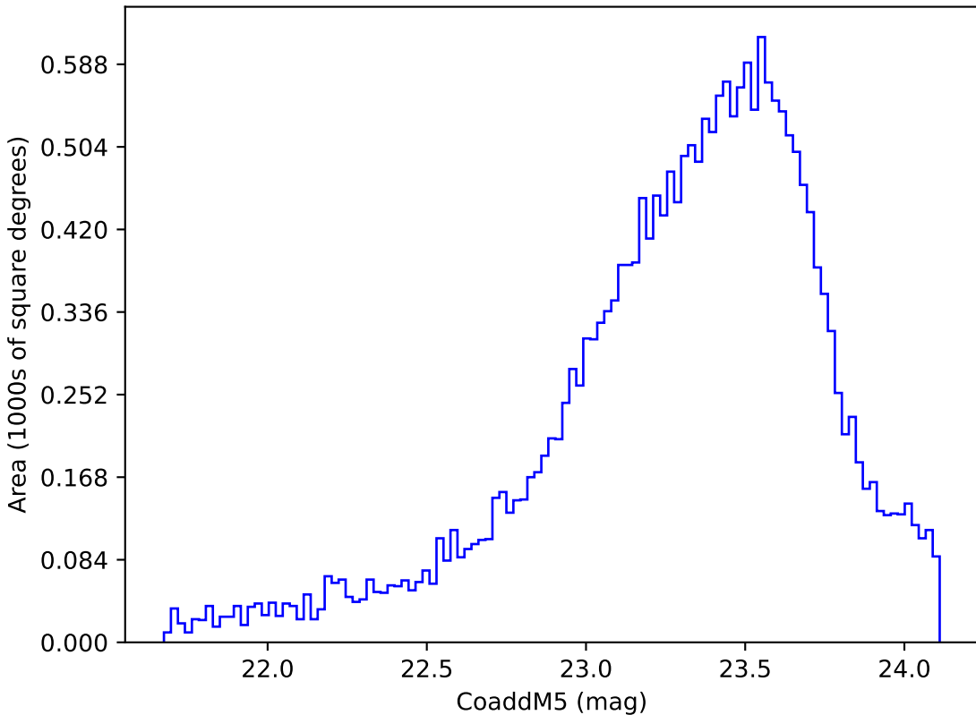
roll_pause_mjdp60_v3.4_10yrs Yr 3-4 y band: CoaddM5
