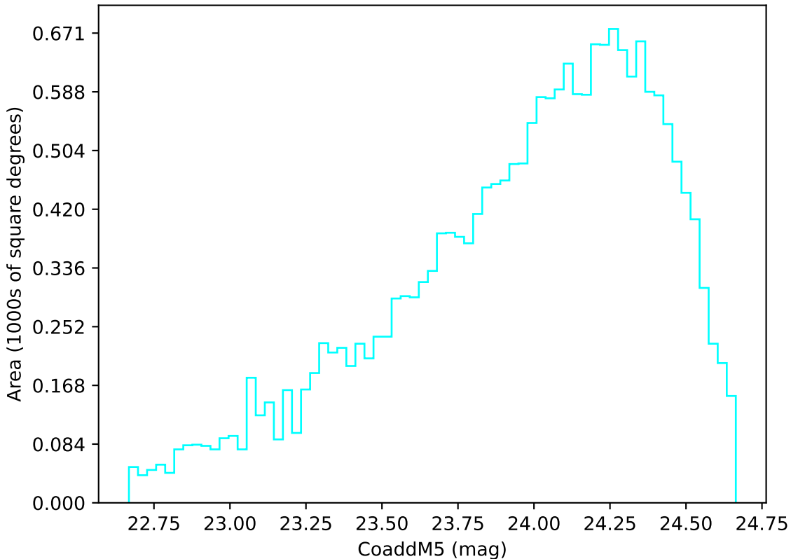
roll_pause_mjdp60_v3.4_10yrs Yr 3-4 u band: CoaddM5
