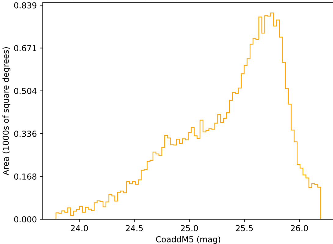
roll_pause_mjdp60_v3.4_10yrs Yr 3-4 r band: CoaddM5
