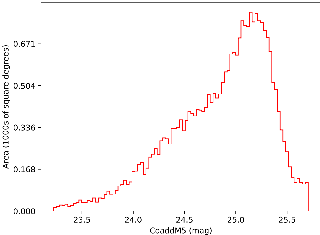
roll_pause_mjdp60_v3.4_10yrs Yr 3-4 i band: CoaddM5
