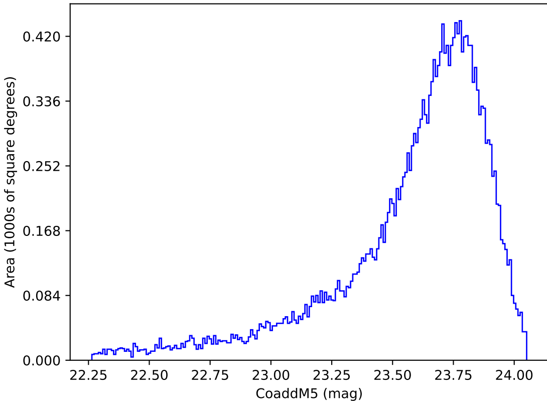
roll_pause_mjdp60_v3.4_10yrs Yr 1 y band: CoaddM5
