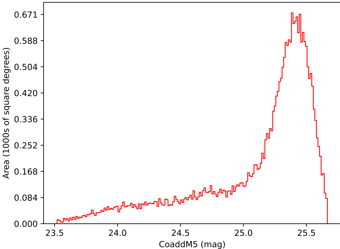
roll_pause_mjdp60_v3.4_10yrs Yr 1 i band: CoaddM5
