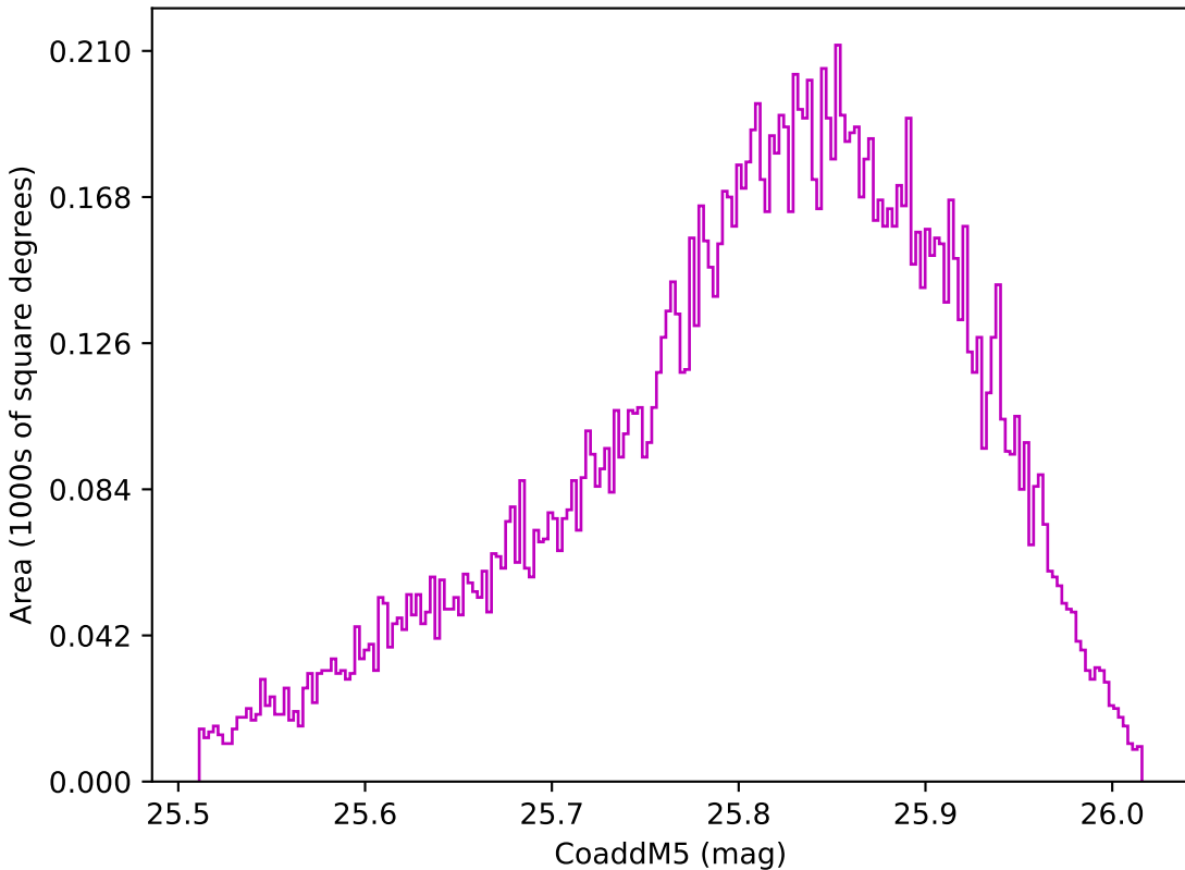
roll_pause_mjdp60_v3.4_10yrs WFD z band: CoaddM5
